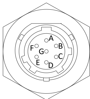
Figure 3.2 Communications Connector
