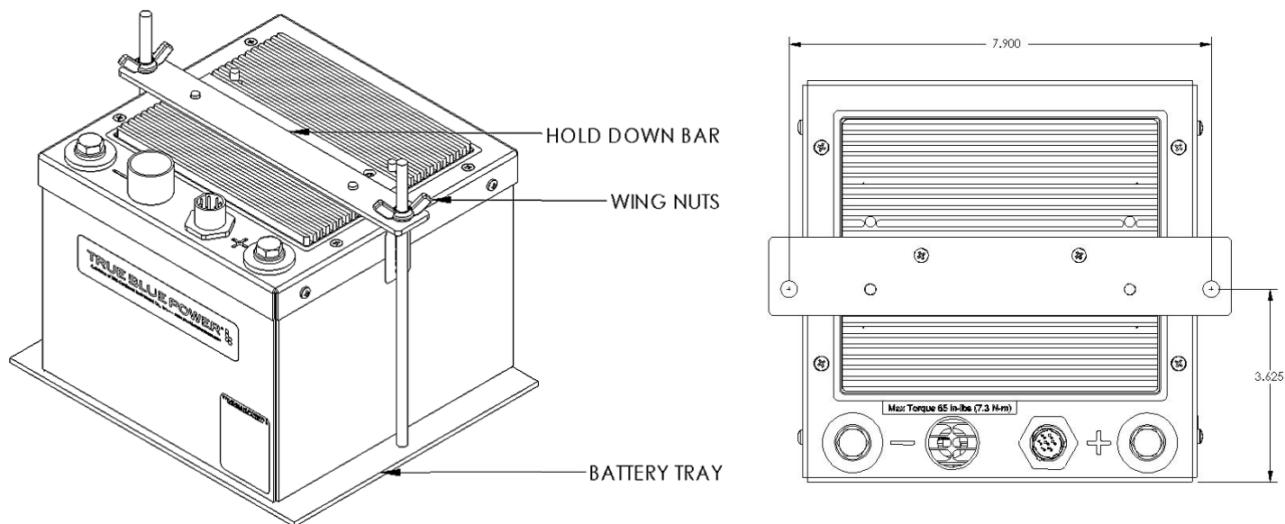
Figure 3.5 Hold-Down Bar Attachment Method
