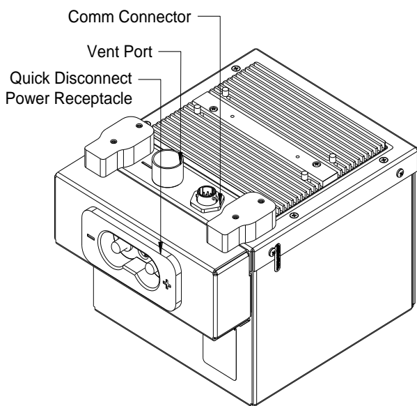
Figure 3.3 Connector Locations
